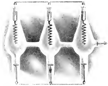
FIG. 45.—Triple valve tube. (C. Andrews.)
